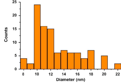
FIG. 7. (Color online) The diameter distribution of \sim 100 bismuth nanorods of Reppert et al. (Ref. 2).
